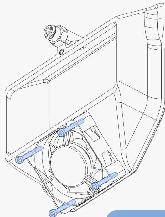
M3x30 SHCS
